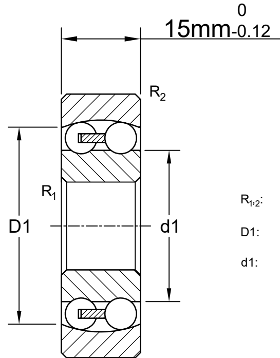
LILY BEARING
