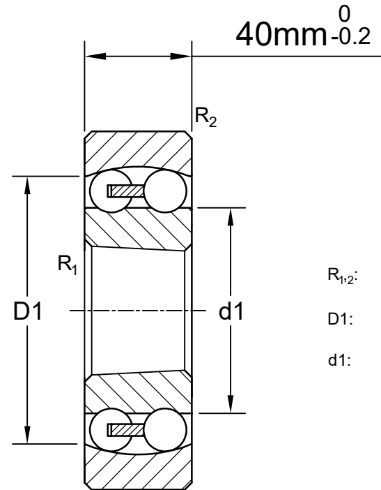
LILY BEARING
