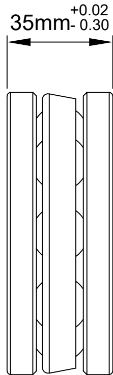
LILY BEARING
