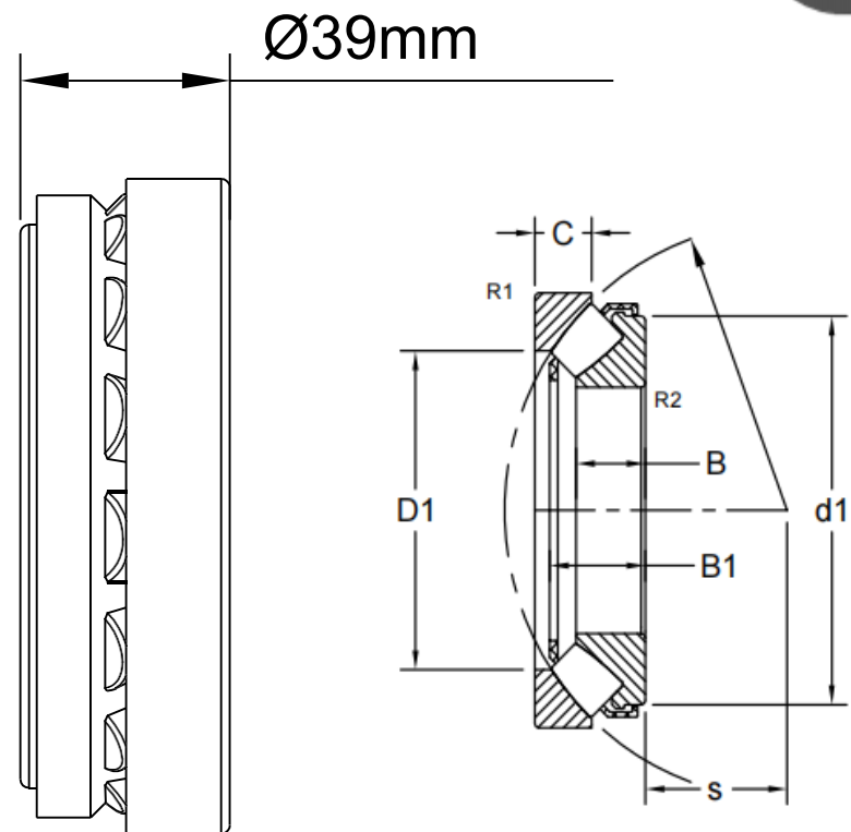
LILY BEARING
