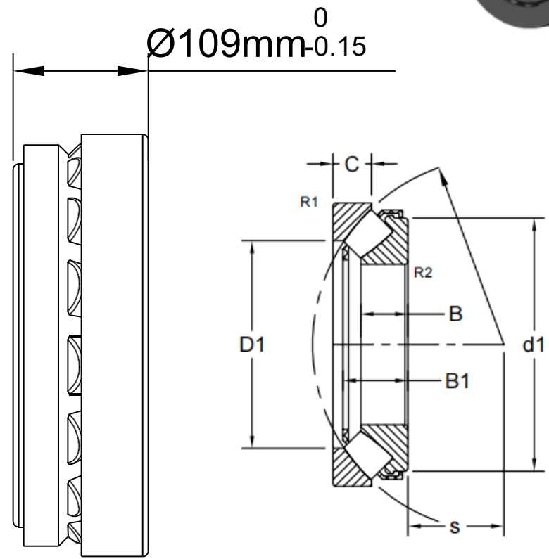
LILY BEARING
