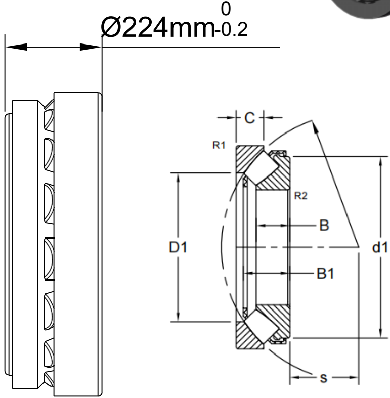
LILY BEARING
