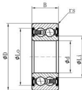
Sealed (RS)
