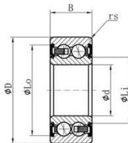
Sealed (RS)
